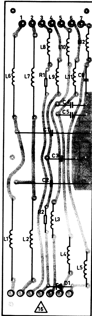
PRINTED CIRCUIT BOARD VIEWED FROM COMPONENT SIDE
