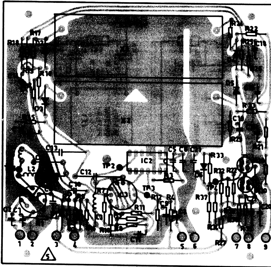
PRINTED CIRCUIT BOARD VIEWED FROM COMPONENT SIDE
